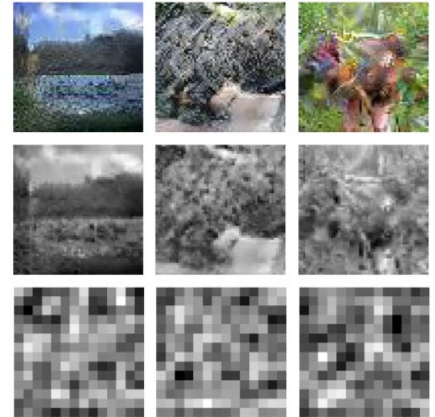
(b) Knockoff data and features
